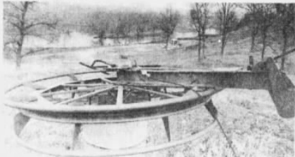
Among the new equipment installed at the ski area is this top pulley for a rope tow on one of the new hills. Three new handle tows were added for the '82-'83 season.
